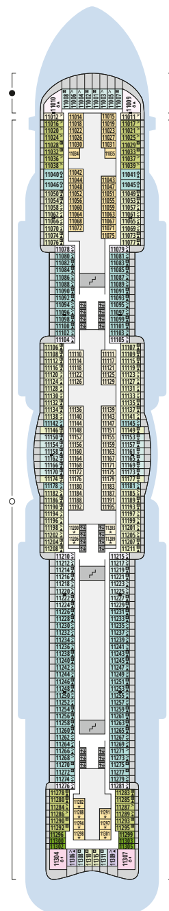
Deck 11
